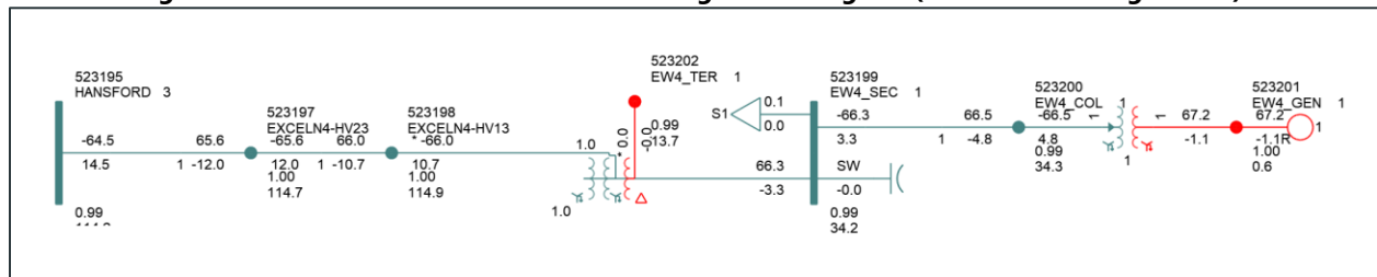
Figure 2: GEN-2002-009 & GEN-2025-SR2 Single Line Diagram (EGF & SGF Configuration)
