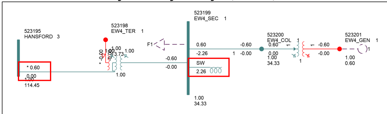
Figure 4: SGF & EGF Single Line Diagram (Shunt Sizes)
