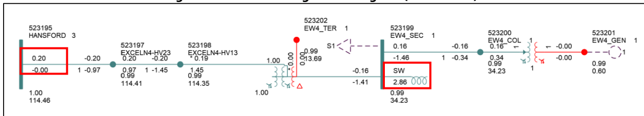
Figure 4: SGF & EGF Single Line Diagram (Shunt Sizes)
