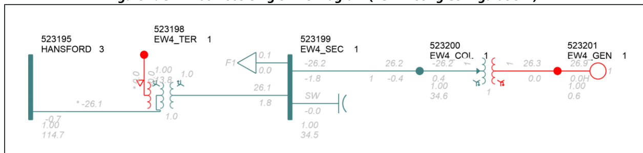
Figure 1: GEN-2002-009 Single Line Diagram (EGF Existing Configuration*)
